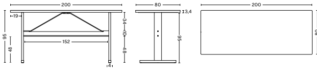
HIGH TABLE WIDTH 200 CM DEPTH 80 CM HEIGHT 95 CM CROSSBAR HEIGHT 48 CM
