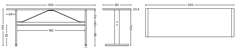
HIGH TABLE WIDTH 250 CM DEPTH 80 CM HEIGHT 105 CM CROSSBAR HEIGHT 58 CM
