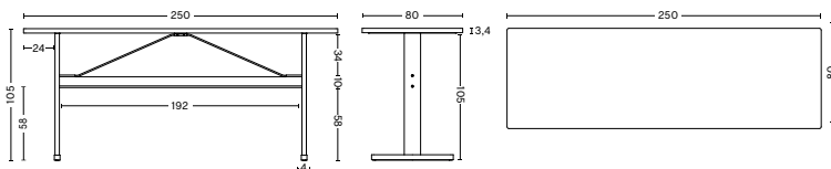
PASSERELLE HIGH TABLE WIDTH 250 CM DEPTH 80 CM HEIGHT 105 CM CROSSBAR HEIGHT 58 CM
