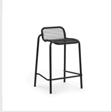
Model: Vig Barstool Design: Simon Legald, 2023 Dimensions: H: 78,5 x W: 51 x D: 45 x SH: 65 cm Specifications: Stackable Material: Double powder coated steel
